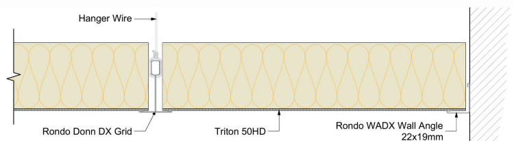
Detail: Triton 50HD ceiling tile suspended on Rondo Donn DX Grid
