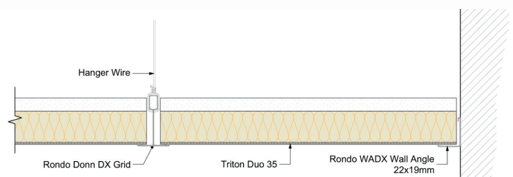
Detail: Triton Duo 35 ceiling tile suspended on Rondo Donn DX Grid
