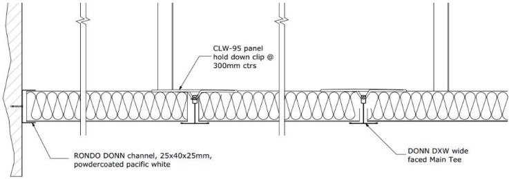
Technical Drawing
