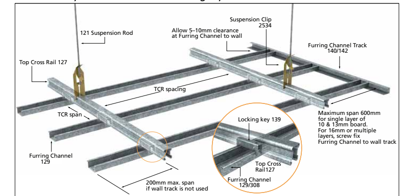
RONDO Key-Lock Concealed Ceiling System
