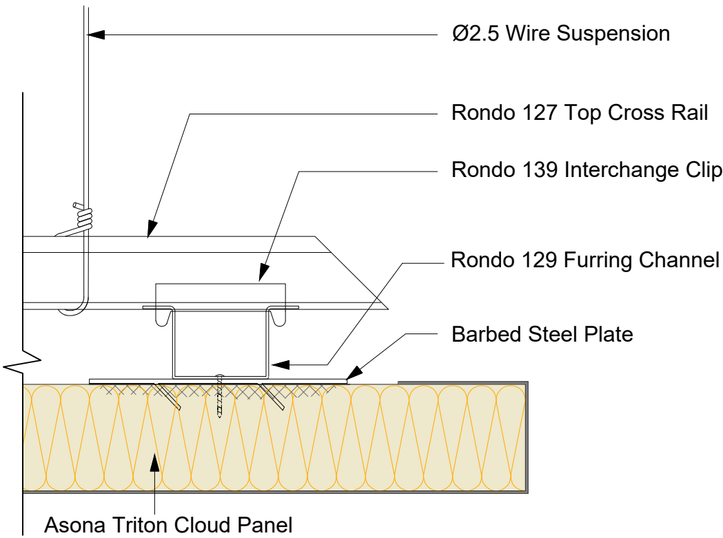
Section View
