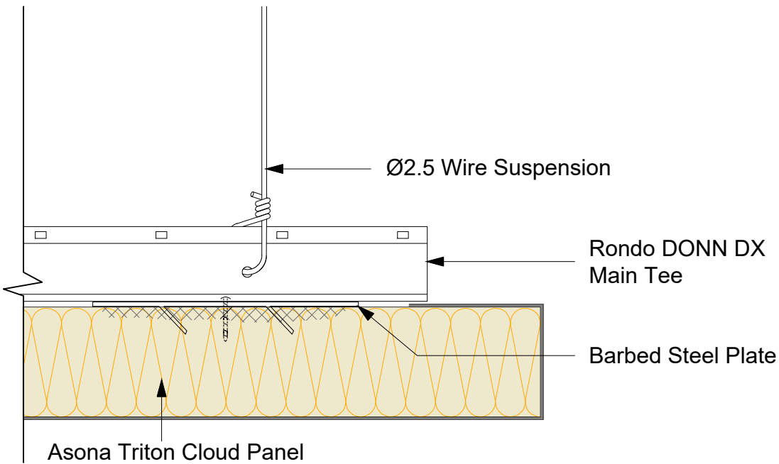
Section View
